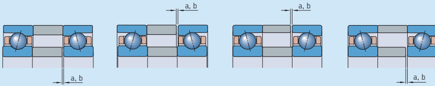
Guideline values for spacer ring width reduction – 718 .. D series
