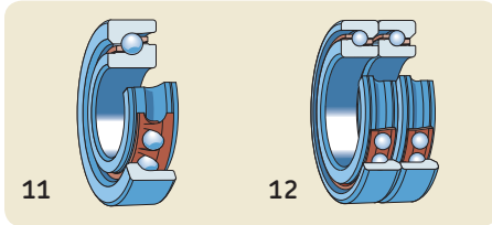
Angular contact thrust ball bearings for screw drives (→ page 22) single direction (BSA and BSD series) (11) , universally matchable for mounting as sets (12) – bearings with seals (13) double direction with seals (BEAS series) (14) – for bolt mounting (BEAM series) (15) cartridge units with a flanged housing (FBSA series) (16)
