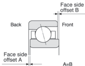
Fig.1.4 Flush grinding
