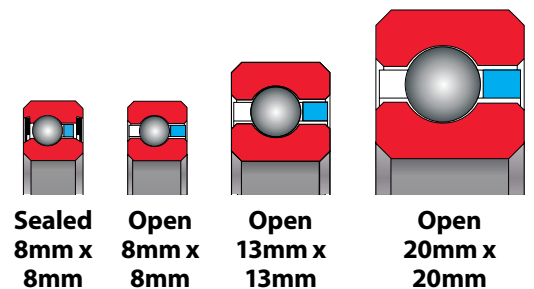
Figure 1-4, Metric Bearings
