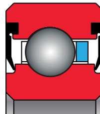
Figure 2-4 Double-Shielded Reali-Slim EA/EB bearing
