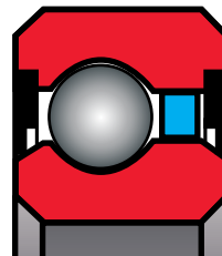
Figure 2-2 Double-Sealed Reali-Slim JU bearing
