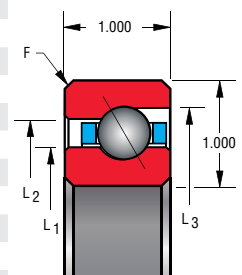
Circular pocket separator 1/2" balls
