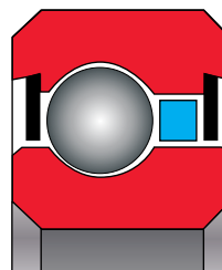
Figure 2-4 Double-Shielded Reali-Slim EA/EB bearing
