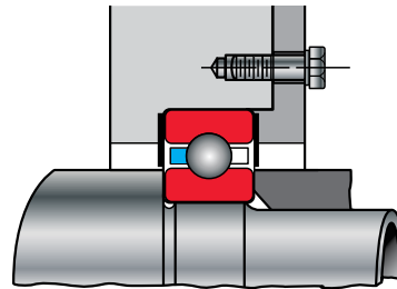
Figure 2-7 Washer Shield From Precision Flat Stock
