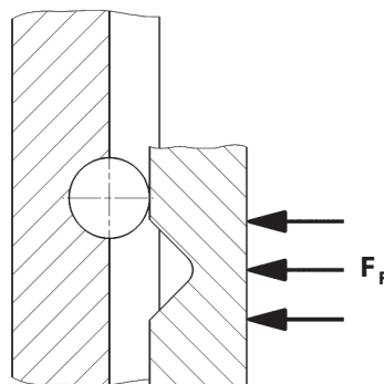
disengaged
