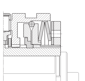
engaged
