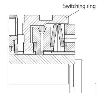
disengaged
