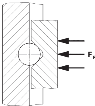
engaged
