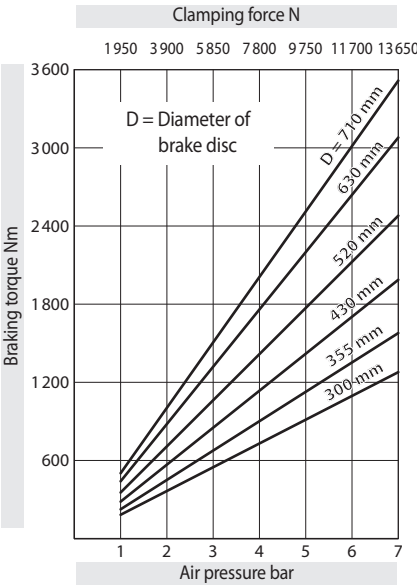
Brake Caliper DV 035 PFM - 655
