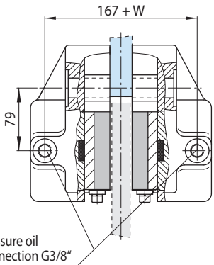
Supply connections
