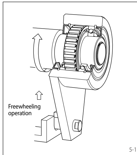
In general, backstops are used where the inner ring freewheels and the stationary held outer ring prevents reverse rotation (figure 5-1).
