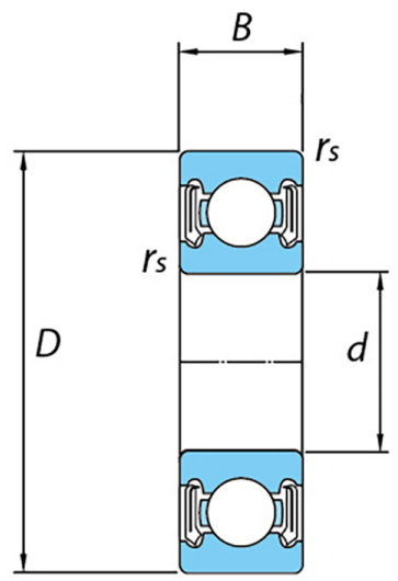
Non-contact sealed type (LLB)
