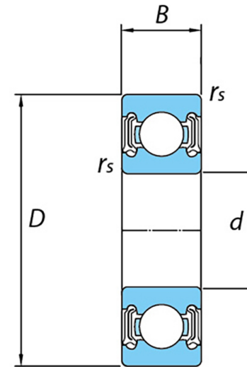
Contact sealed type (LLU)
