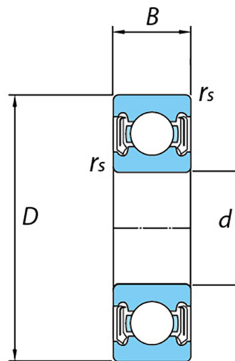
Non-contact sealed type (LLB)
